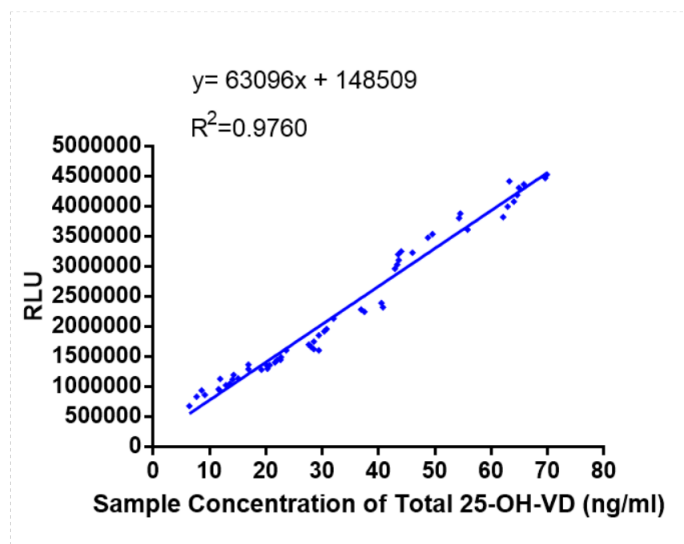
Figure 4. Clinical comparative analysis; As can be seen from the figure above, Detection employing 25-OH-VD sandwich antibodies validated by an enzymatic chemiluminescence platform using an R² of 0.9760, the data demonstrated strong consistency using mass spectrometry (LC-MS/MS).
